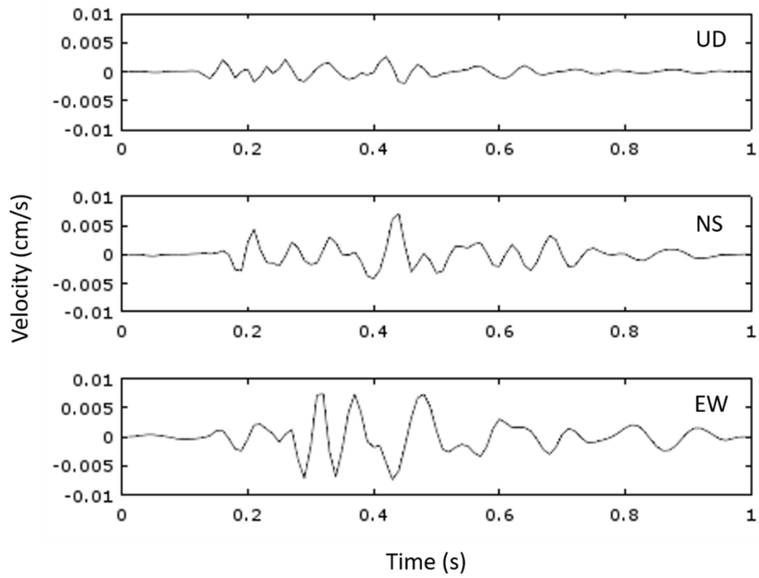
Figure-1 Seismic waveforms in three components with an impact of a hammer.
